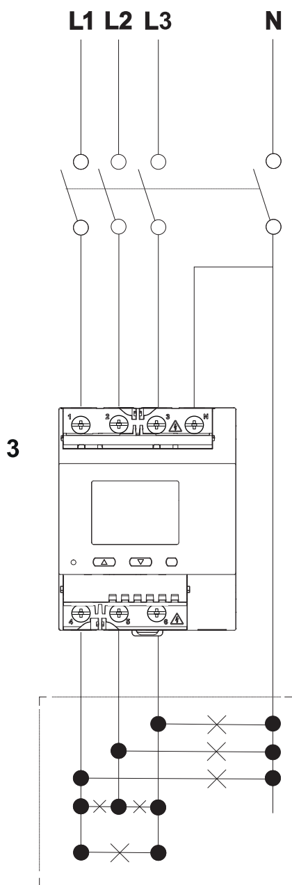
Fig. 3 Three-phase with neutral (4-wire)
